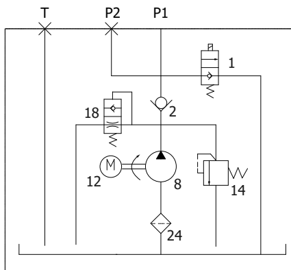
Hydraulic Schematic
