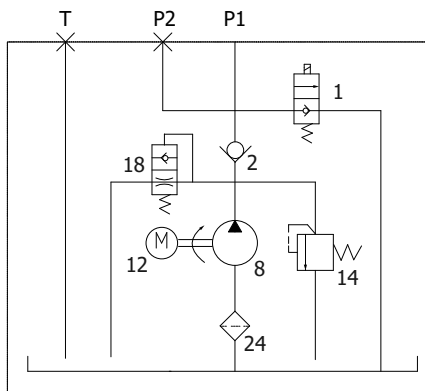
Hydraulic Schematic
