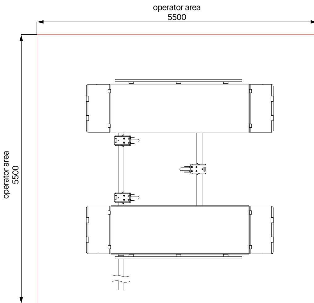
Foundation plan above-ground
