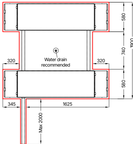
Foundation plan underfloor
